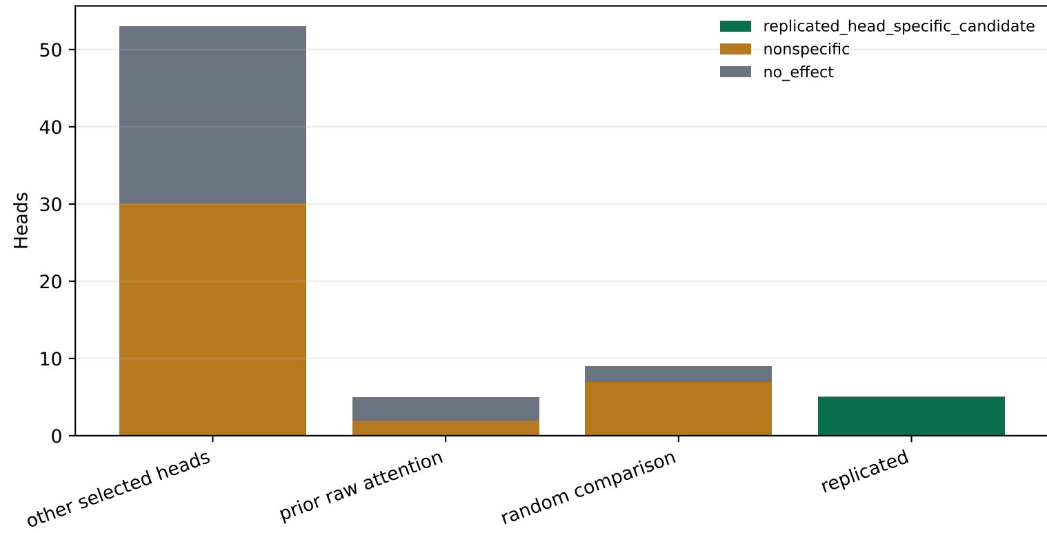
Outcome by candidate provenance
