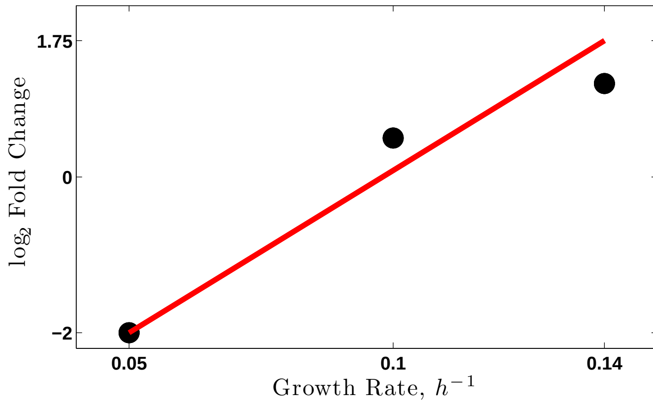
Poor Fit & Monotonic: Grade 2
