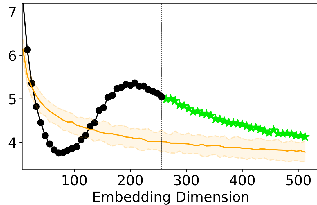
Cutoff=100%
