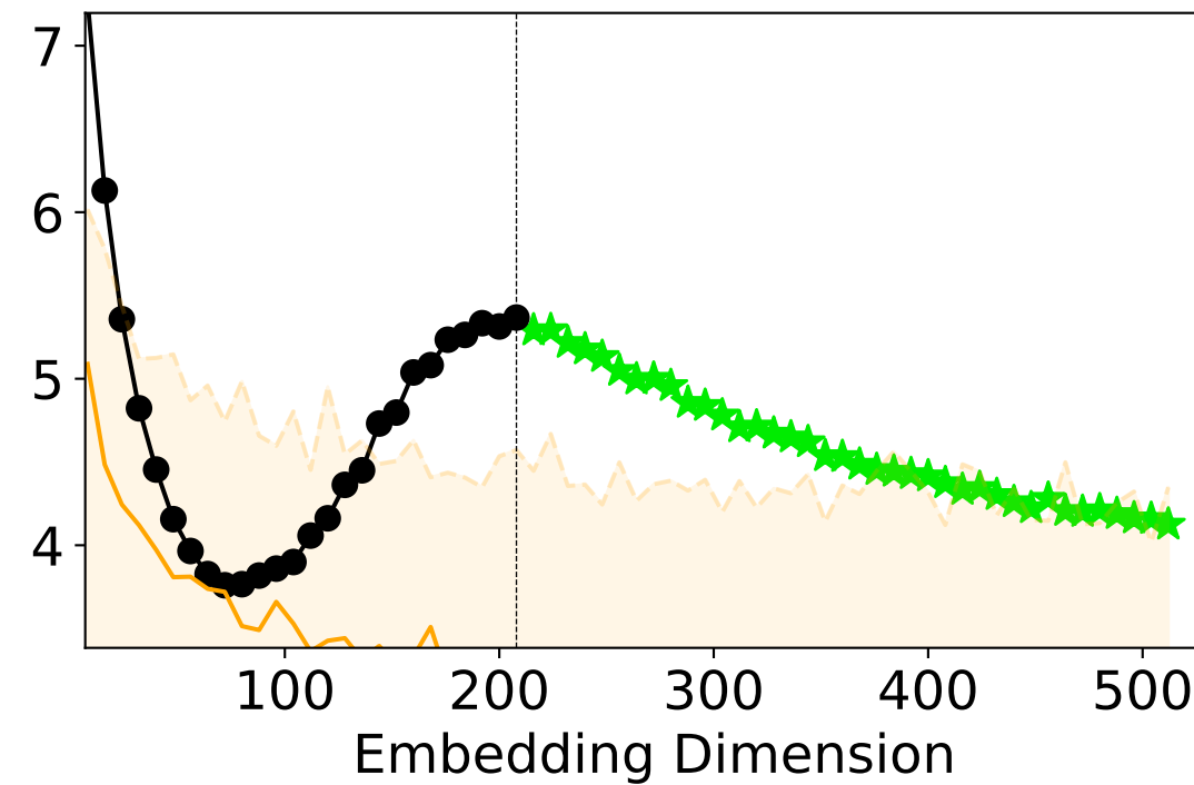
Cutoff=80%
