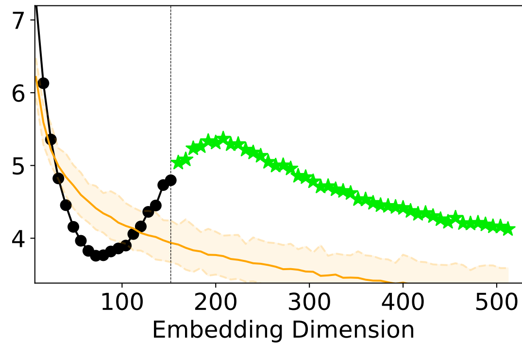
Cutoff=60%
