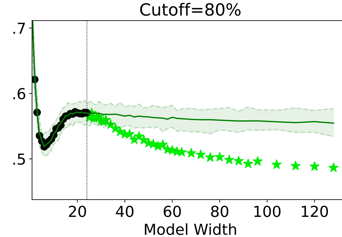
cifar10-mcnn-p20-sgd-rep4
