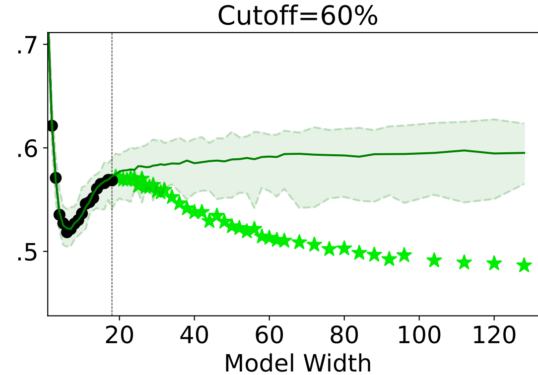
cifar10-mcnn-p20-sgd-rep4
