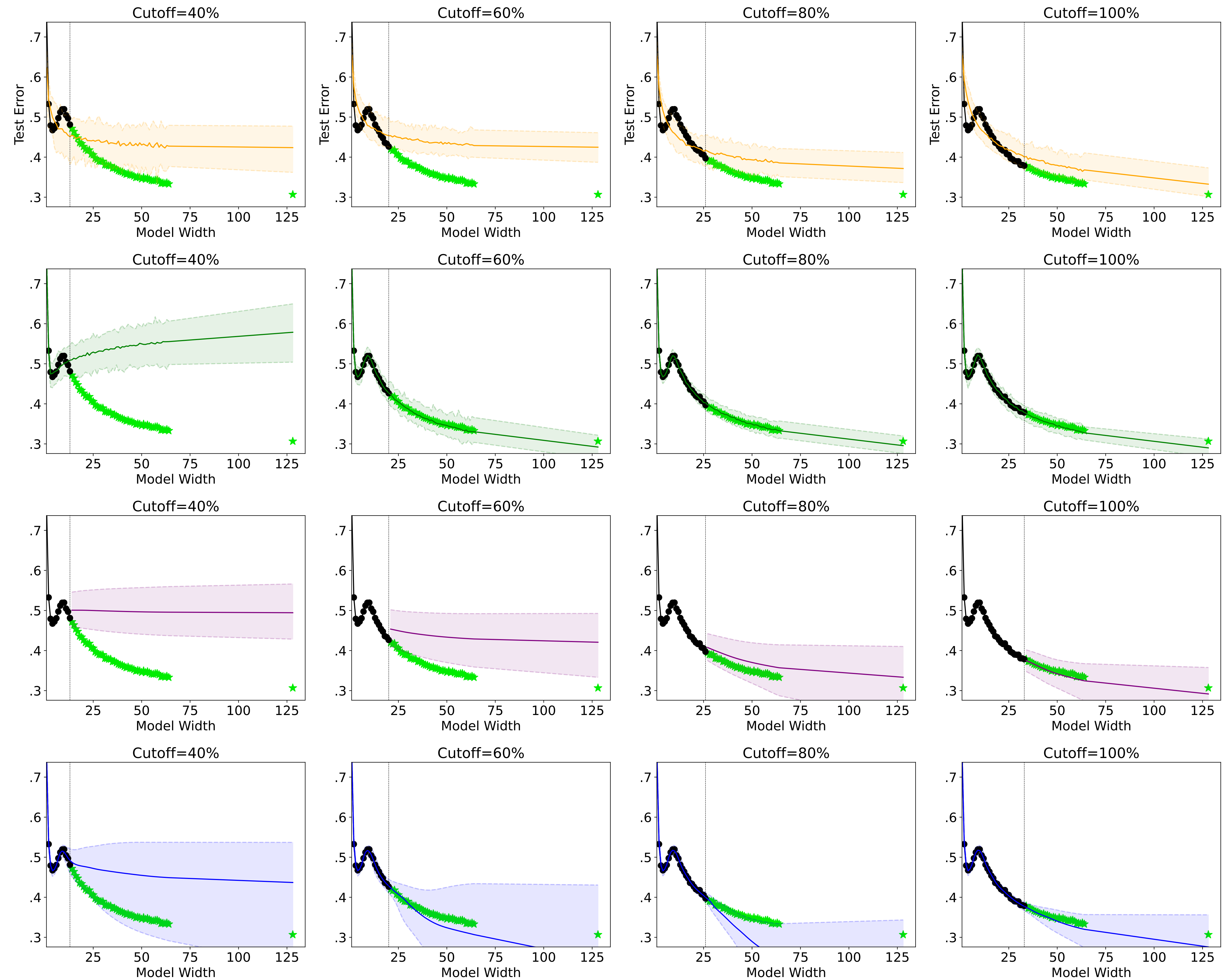
cifar10-mcnn-noaug-sgd
