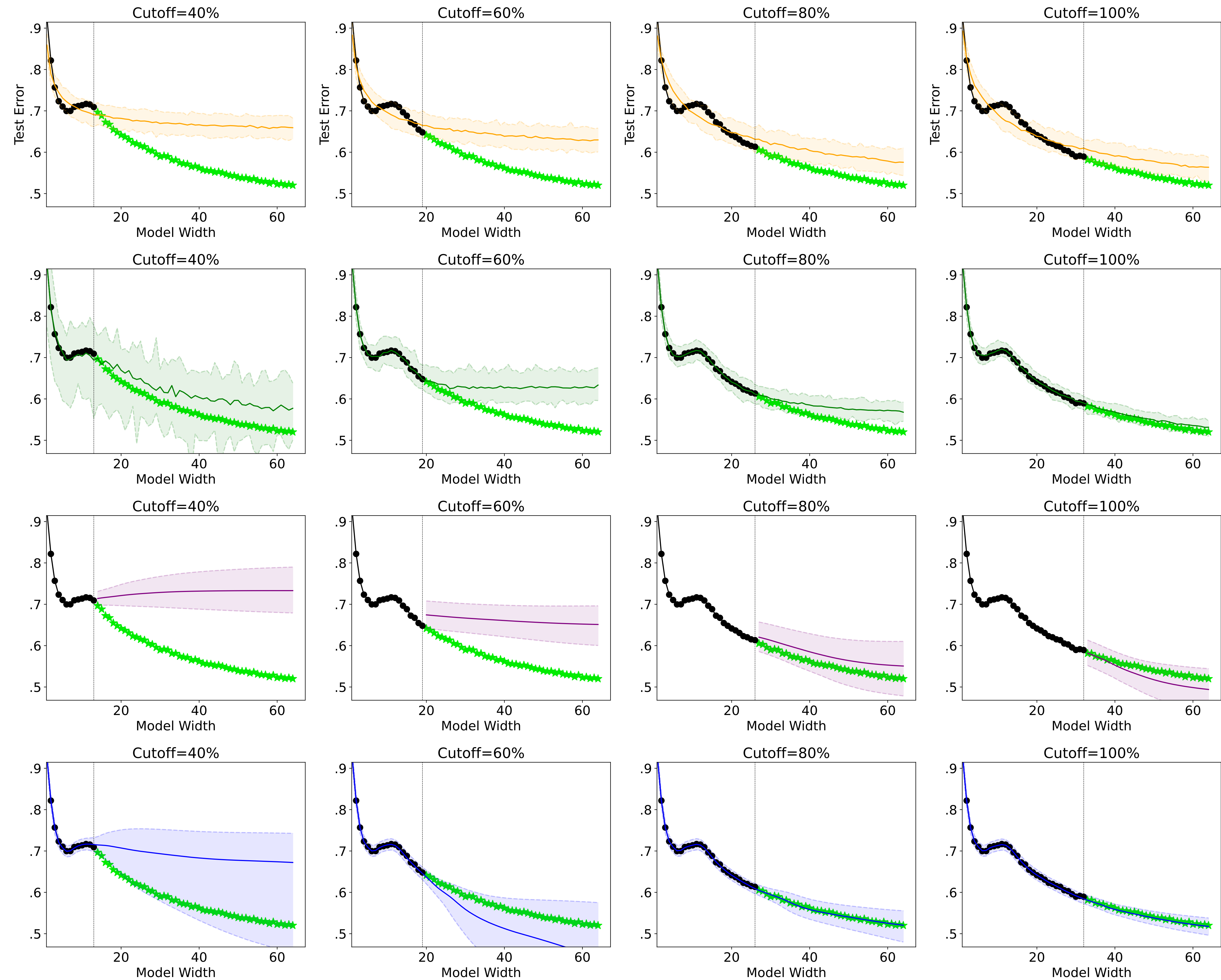
pct-cifar100-mcnn-p0-sgd-noaug-reps
