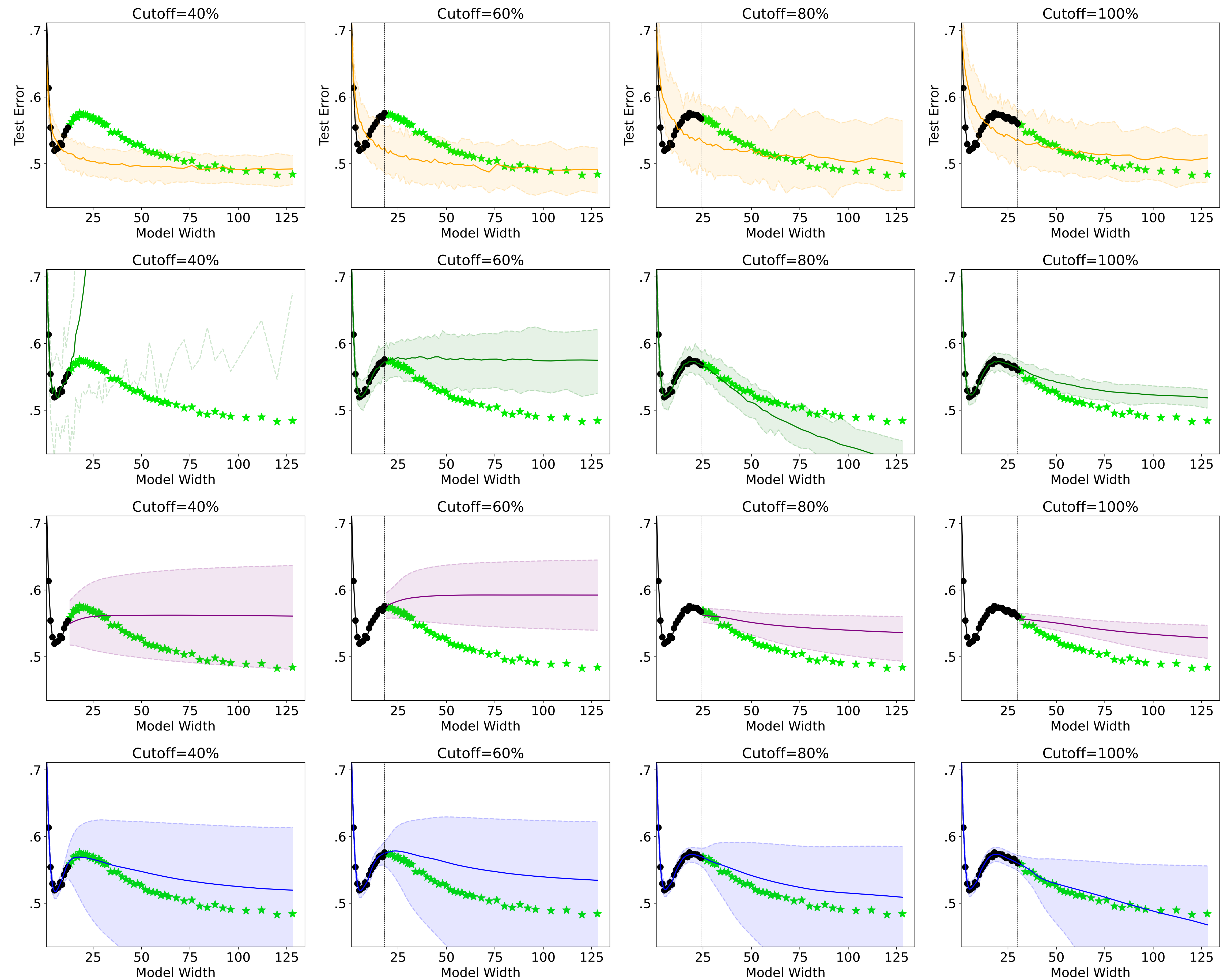
cifar10-mcnn-p20-sgd
