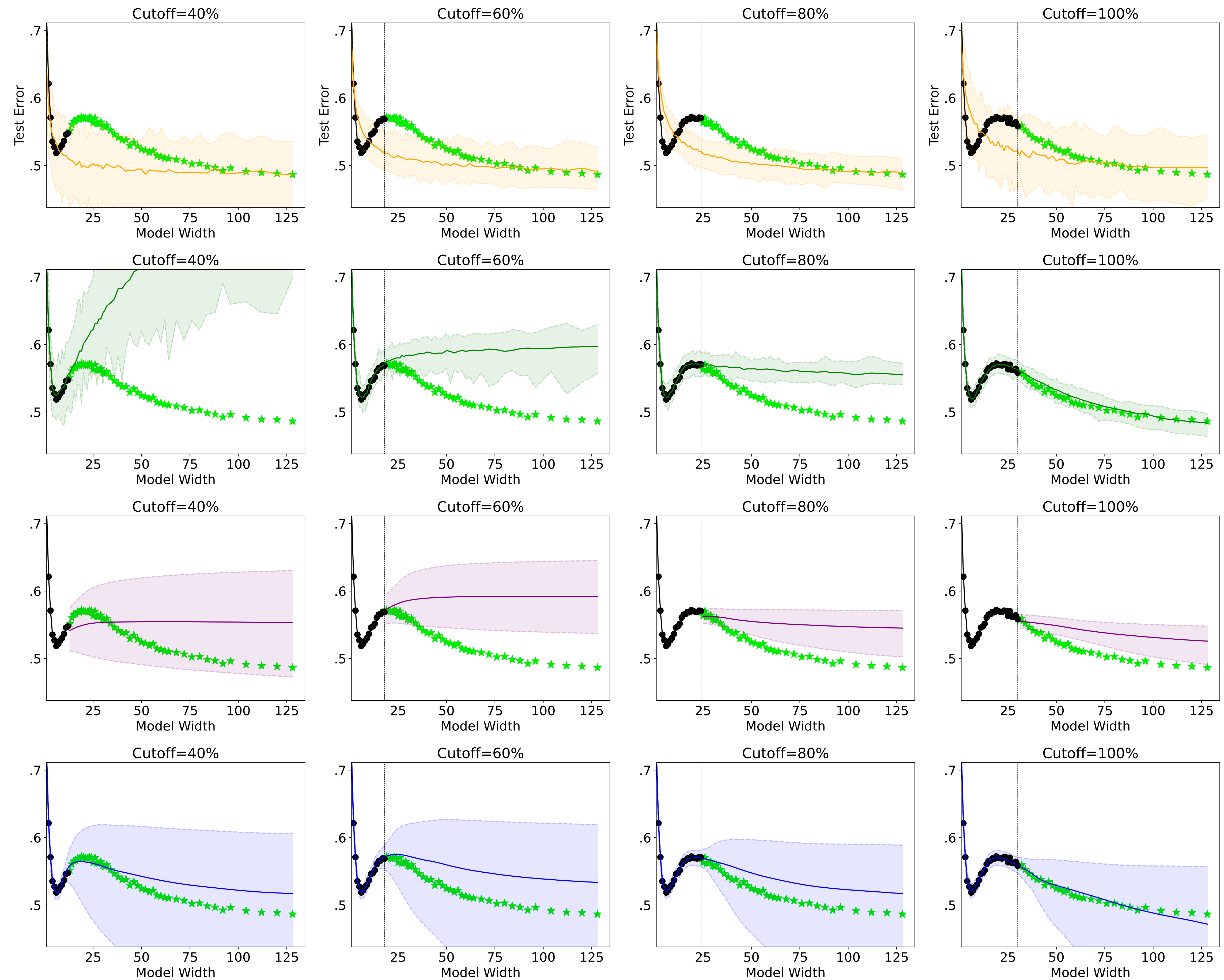
cifar10-mcnn-p20-sgd-rep4
