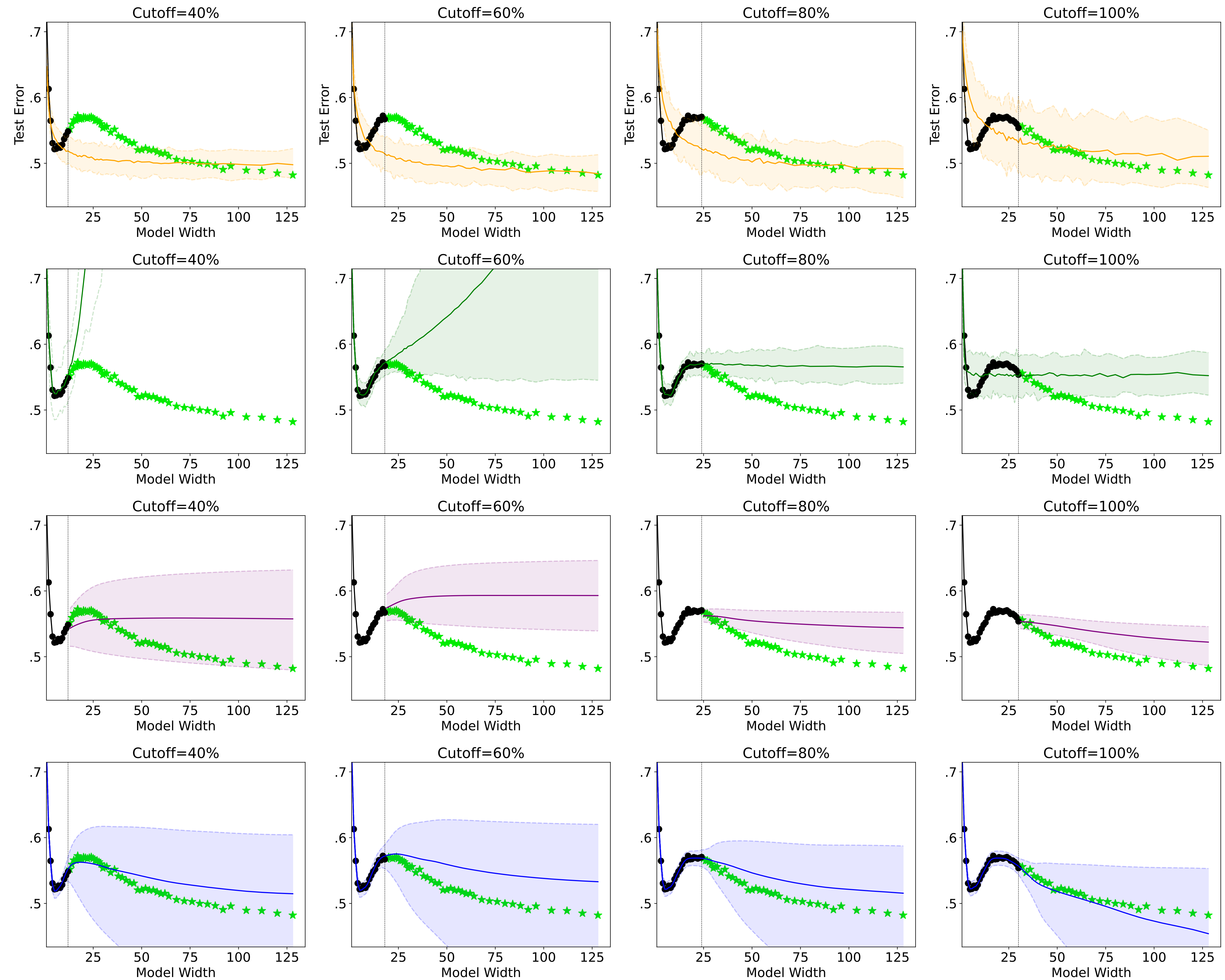
cifar10-mcnn-p20-sgd-rep5
