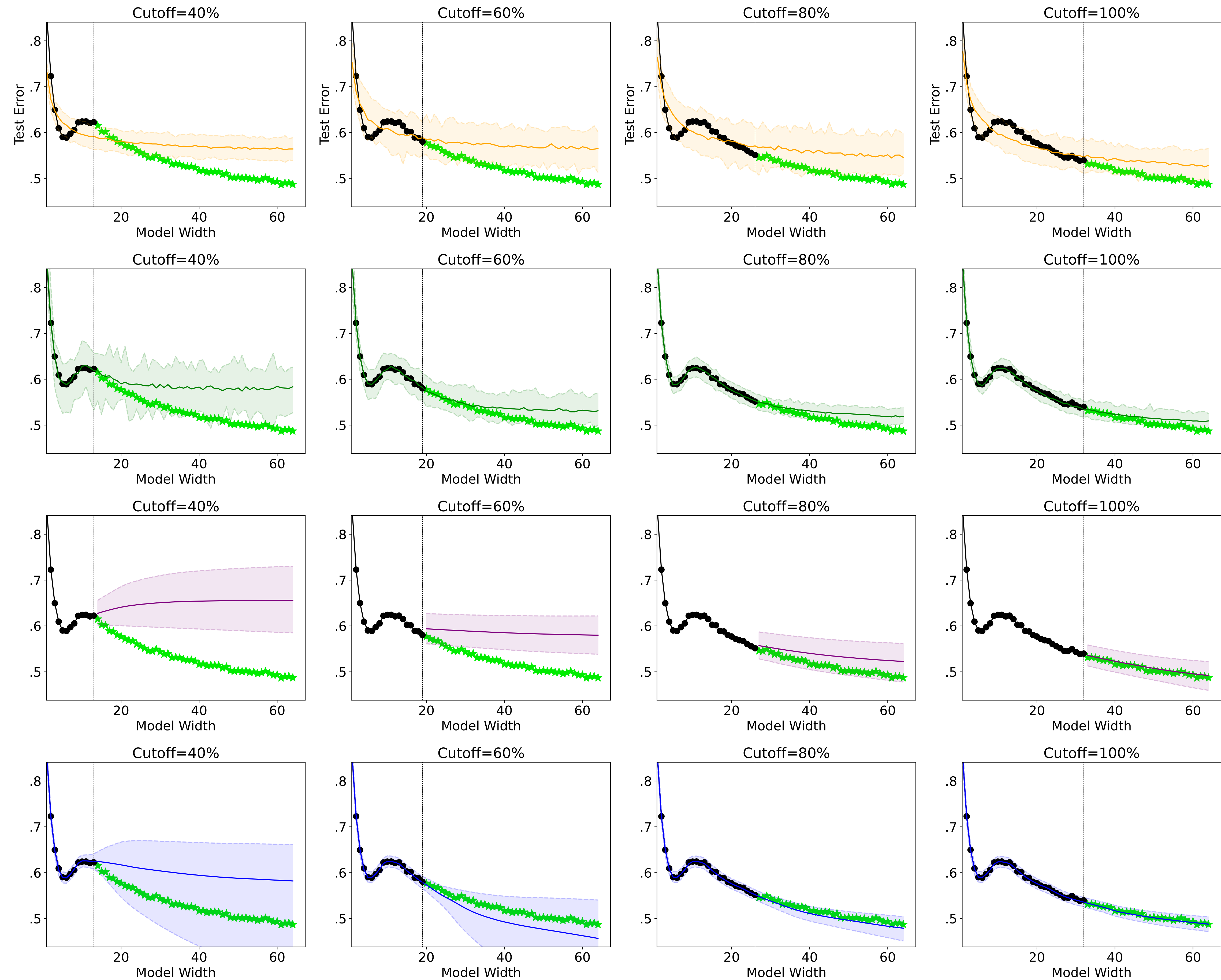
cifar100-resnet18k-50k-adam
