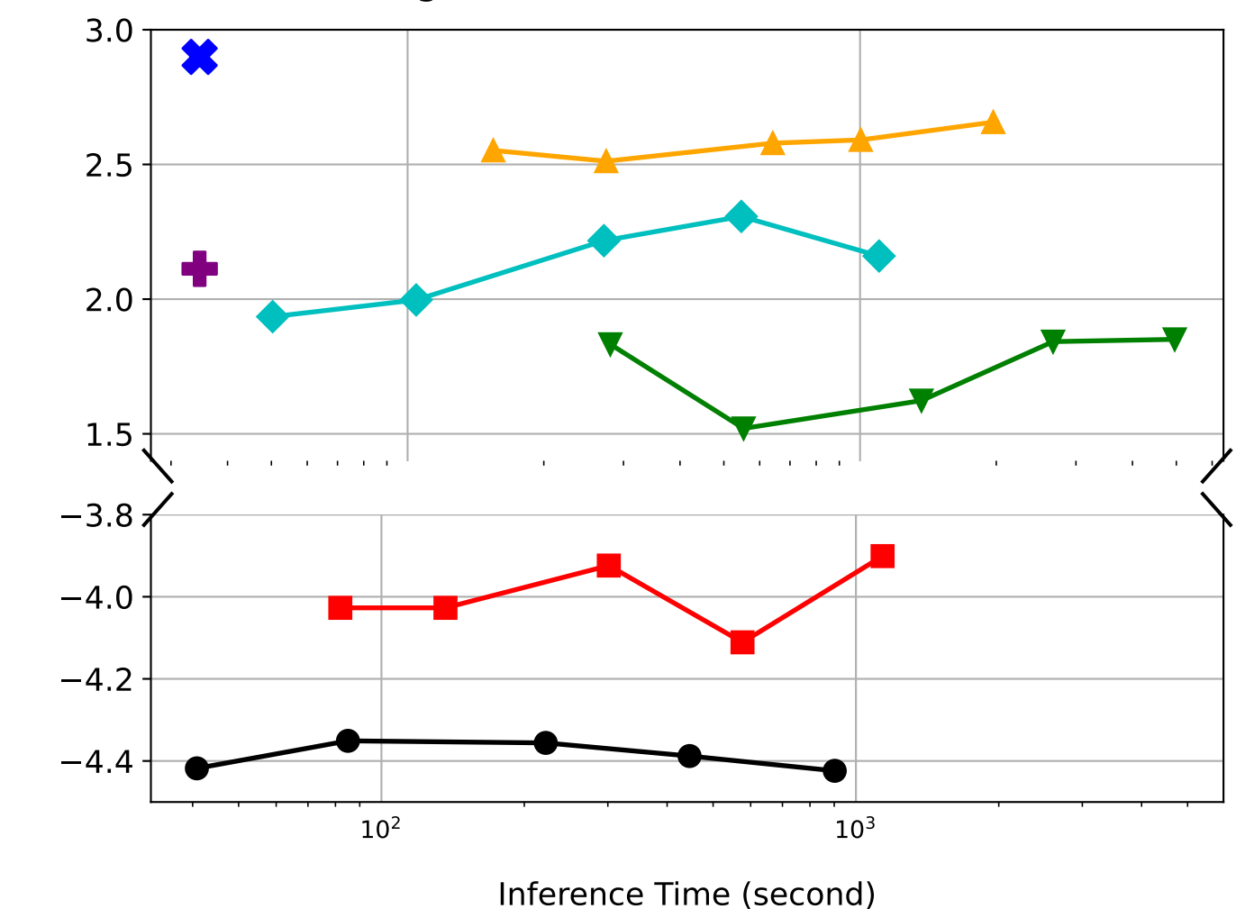
Log-likelihood vs. Inference Time
