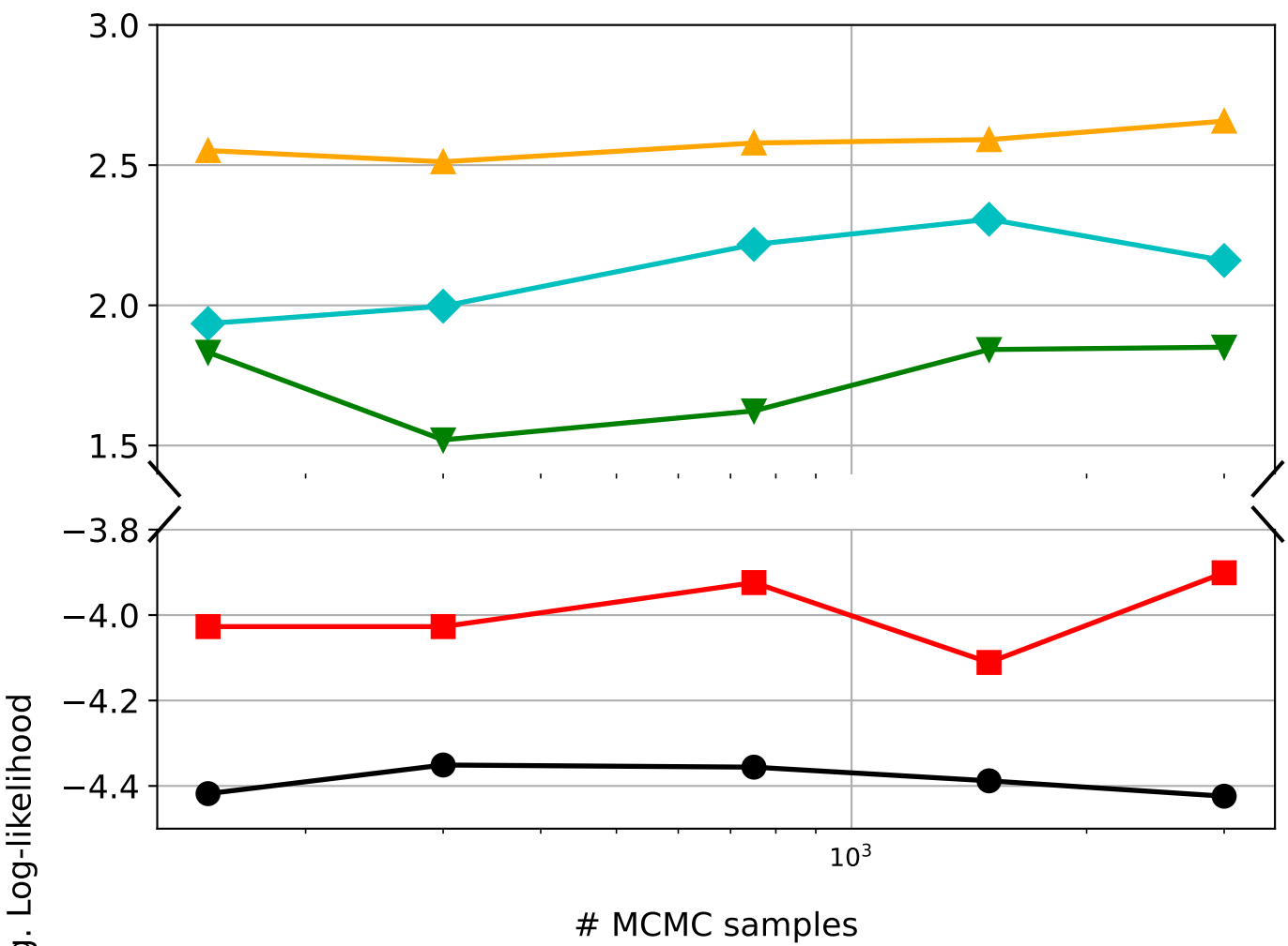
Log-likelihood vs. # MCMC samples
