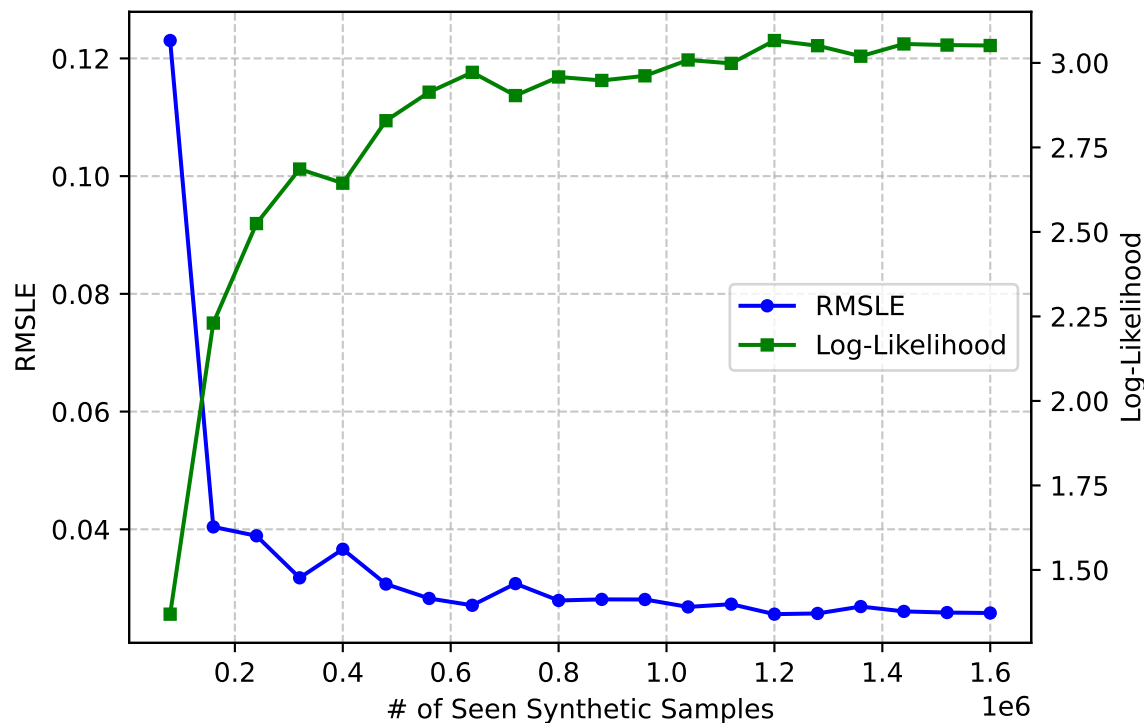
Test RMSLE & LL for IC, NLP, Nano and DD
