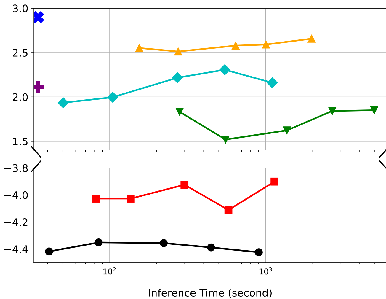
Log-likelihood vs. Inference Time
