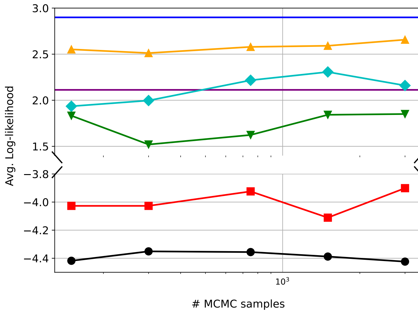
Log-likelihood vs. # MCMC samples
