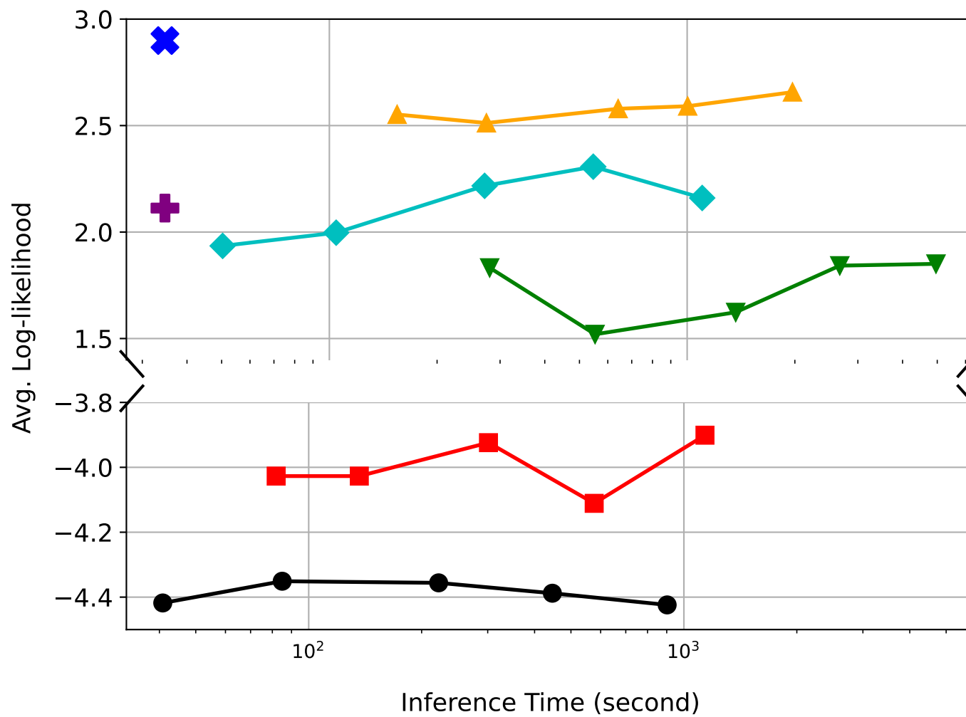
Log-likelihood vs. Inference Time
