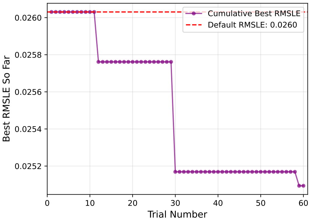
Cumulative Best Error over Trials
