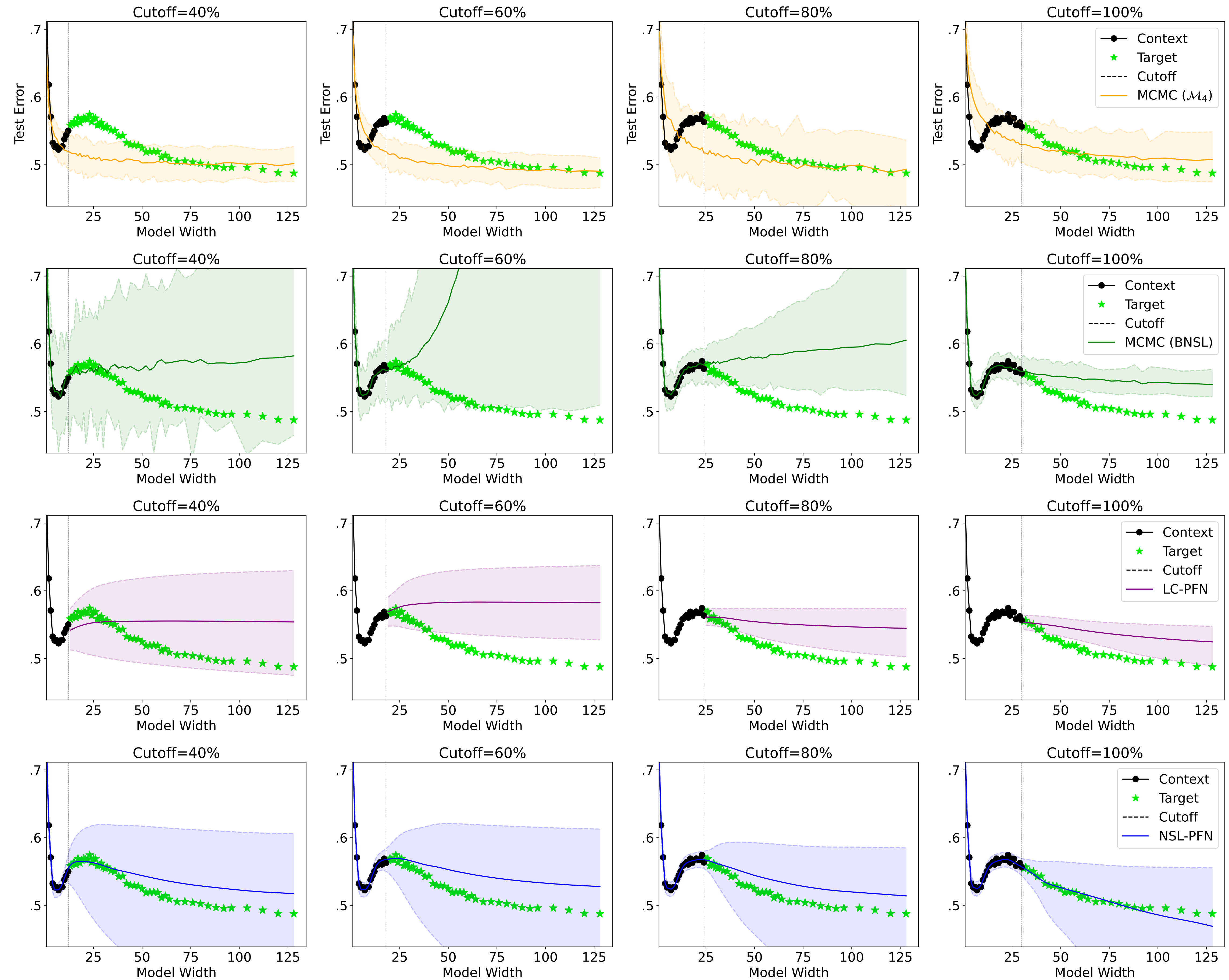
cifar10-mcnn-p20-sgd-rep3
