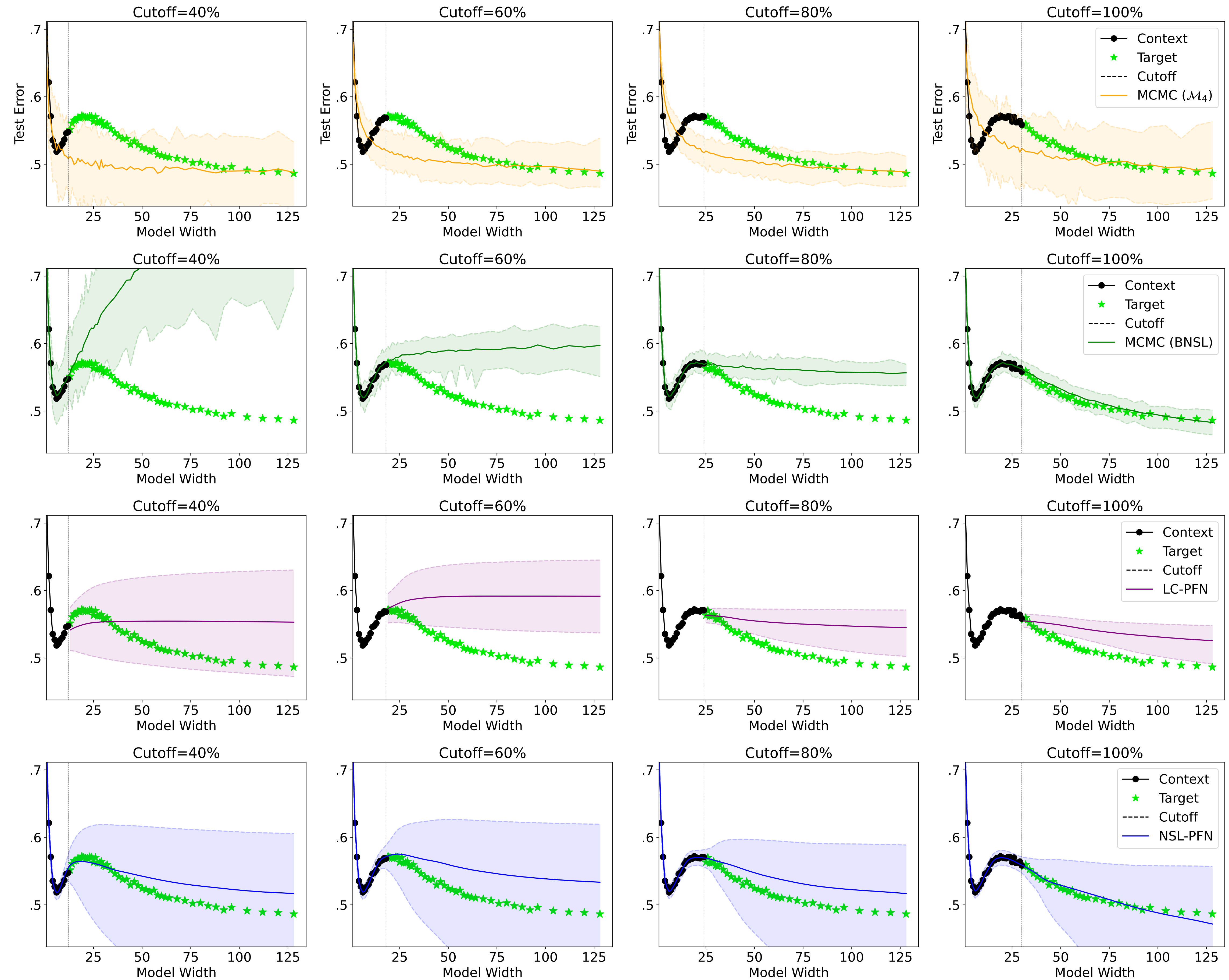
cifar10-mcnn-p20-sgd-rep4
