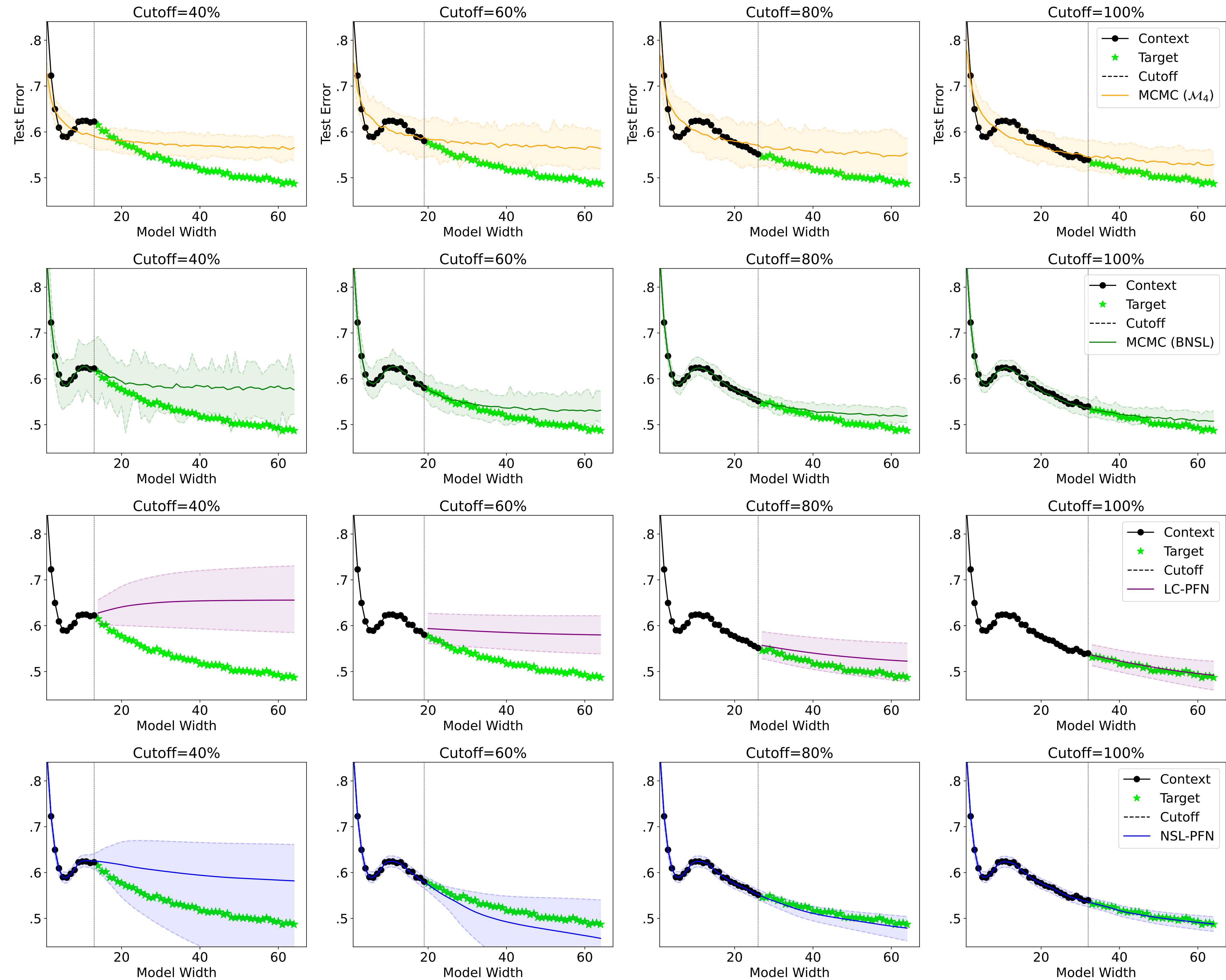
cifar100-resnet18k-50k-adam
