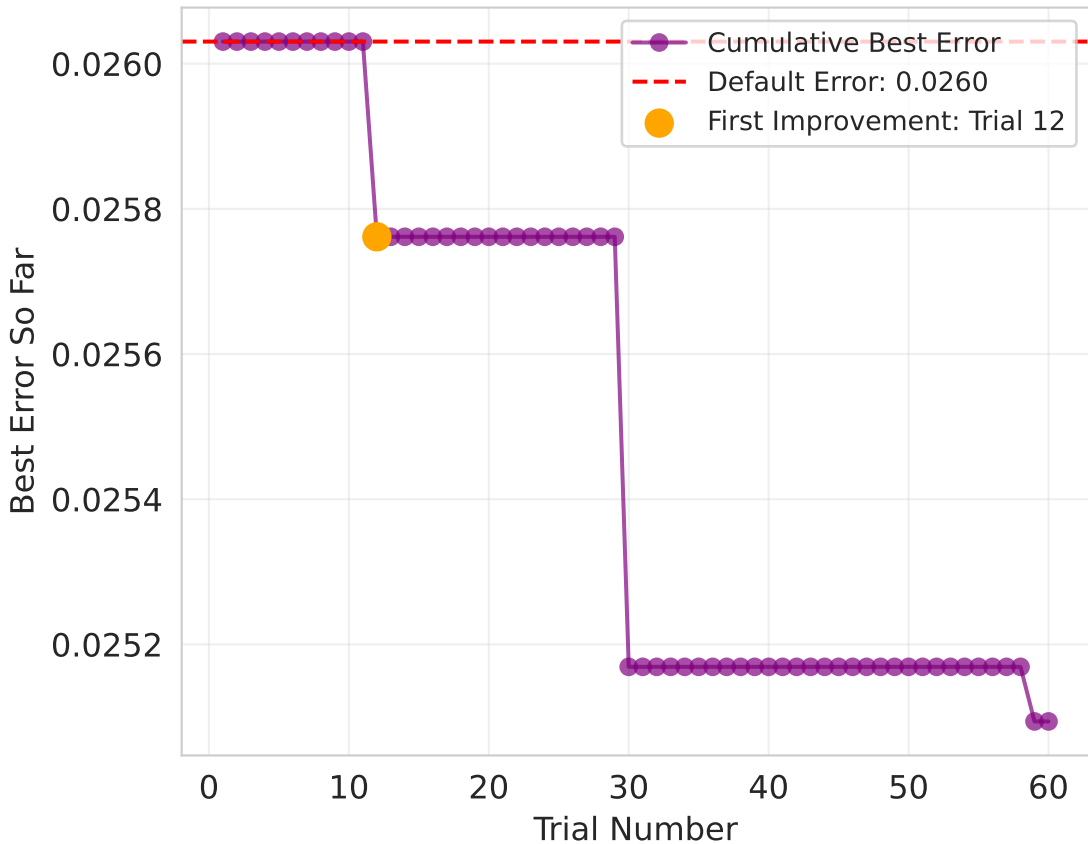
Cumulative Best Error over Trials
