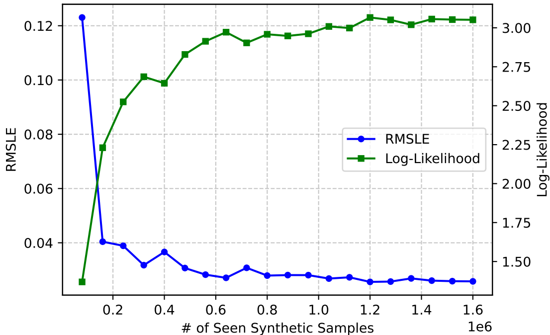
Test RMSLE & LL for IC, NLP, Nano and DD
