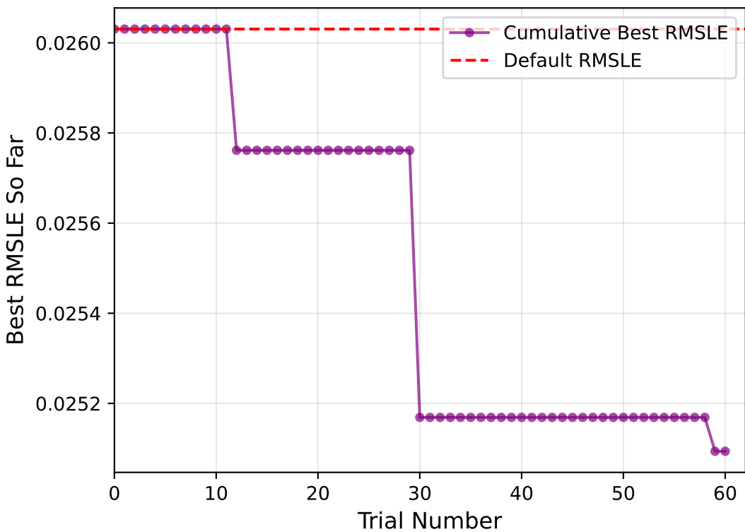
Cumulative Best Error over Trials
