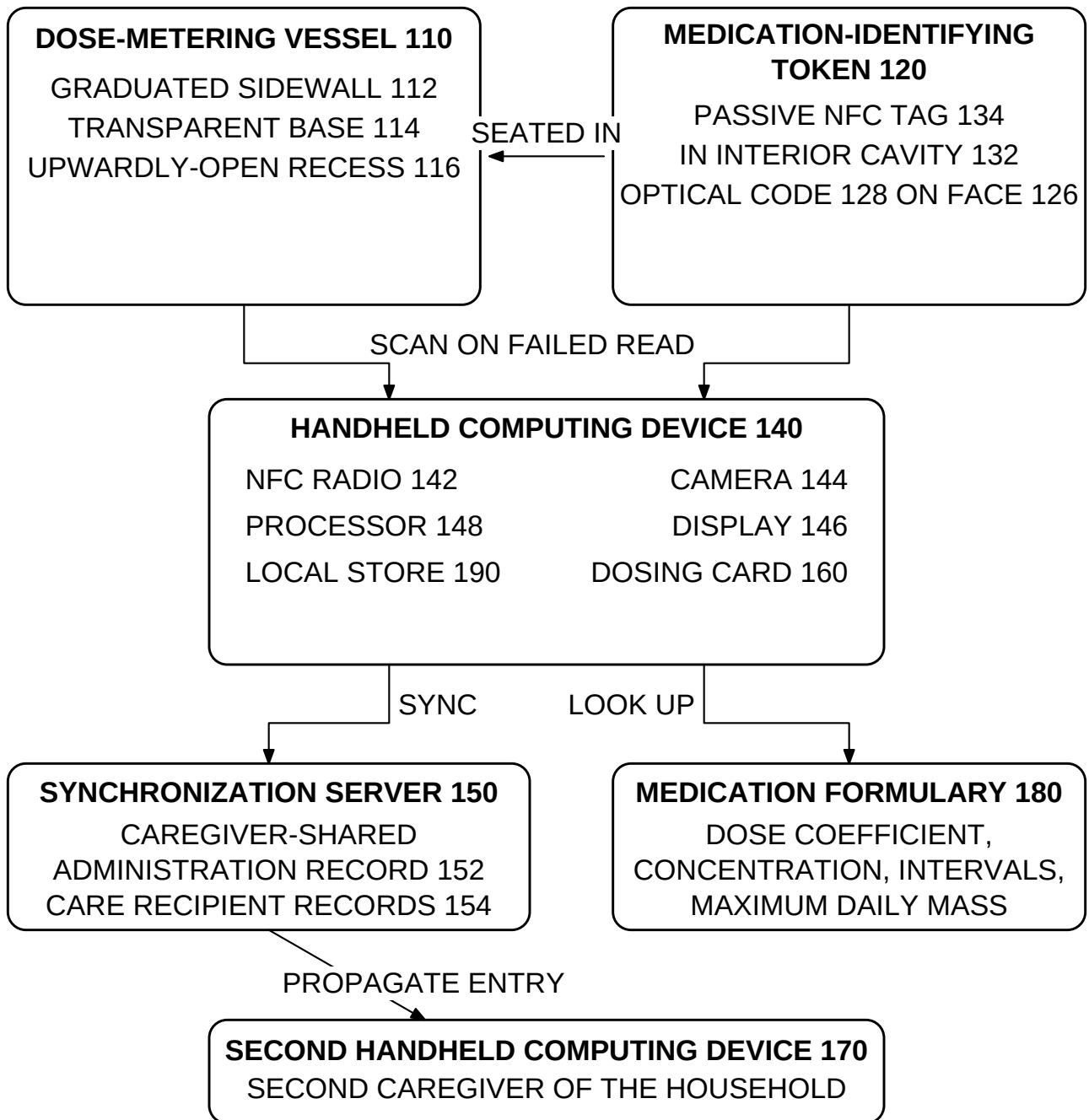
FIG. 5 MEDICATION DOSING SYSTEM 100
