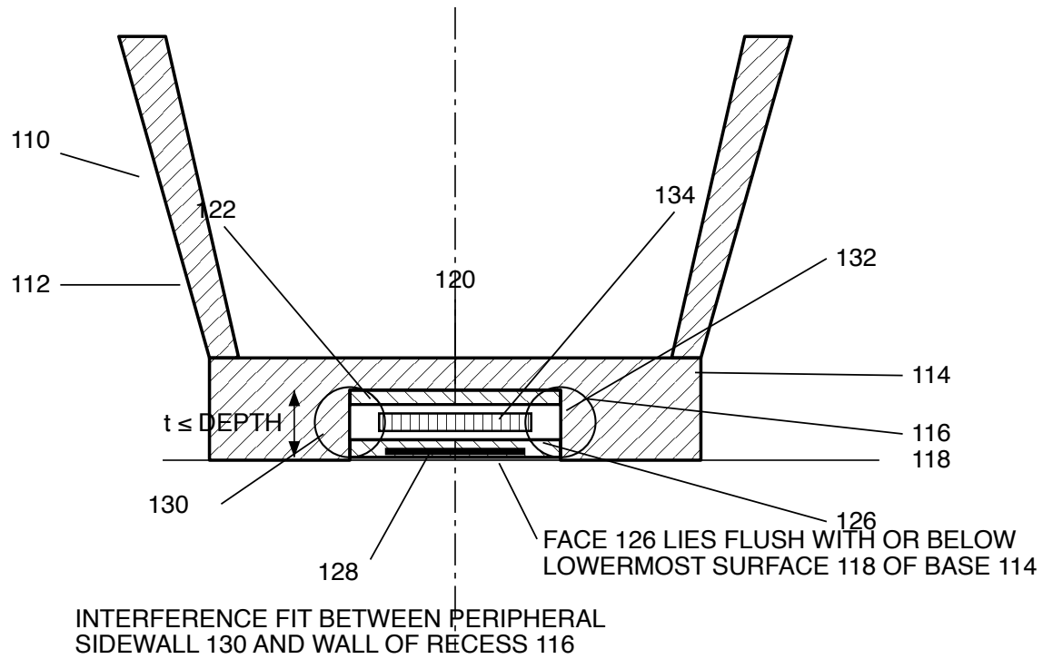
FIG. 2 SECTIONAL VIEW — TOKEN 120 SEATED IN RECESS 116
