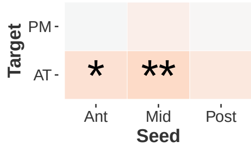
Encode Sham
