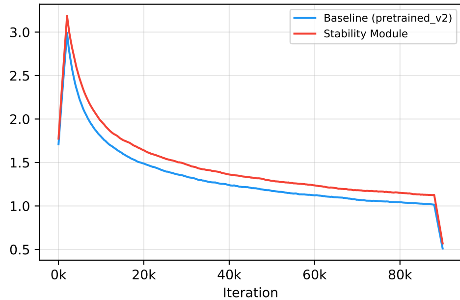
Dice Loss
