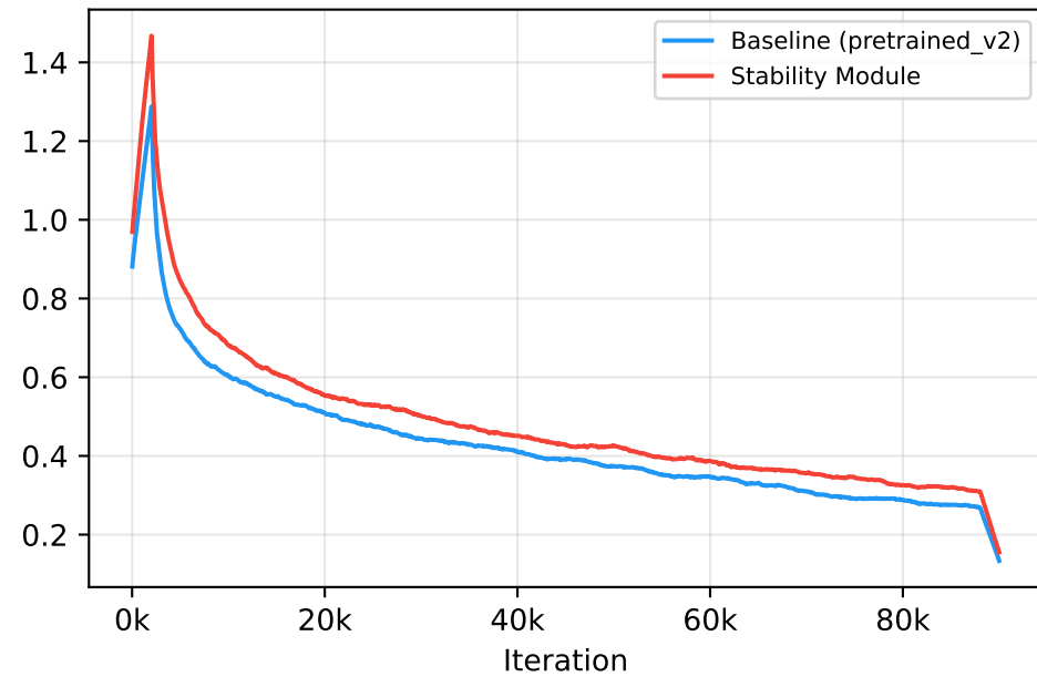
CE Loss
