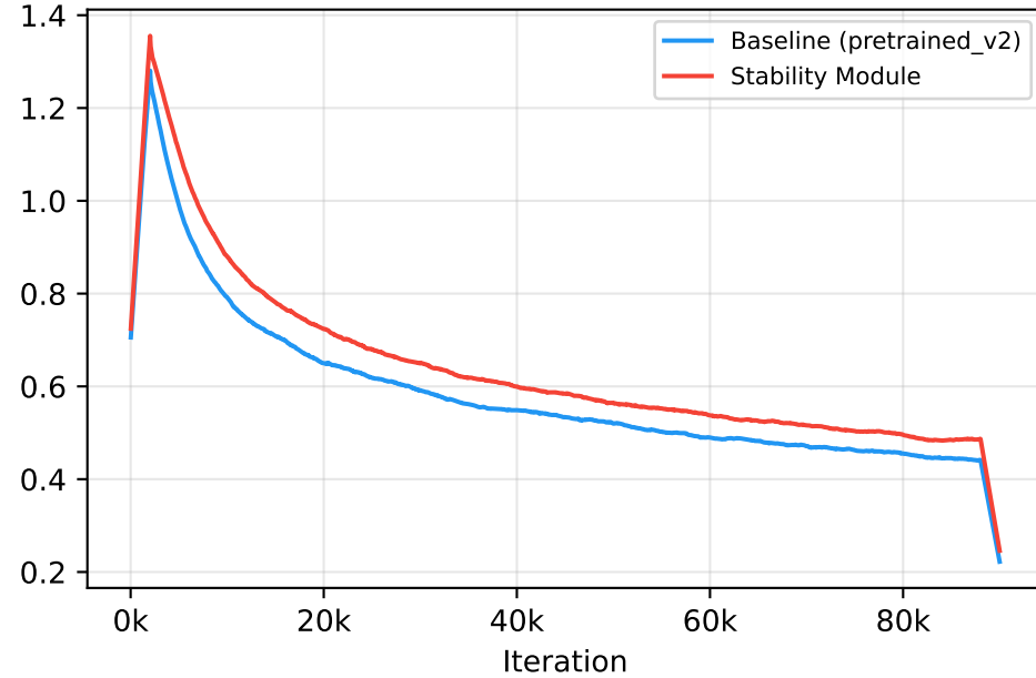
Mask Loss
