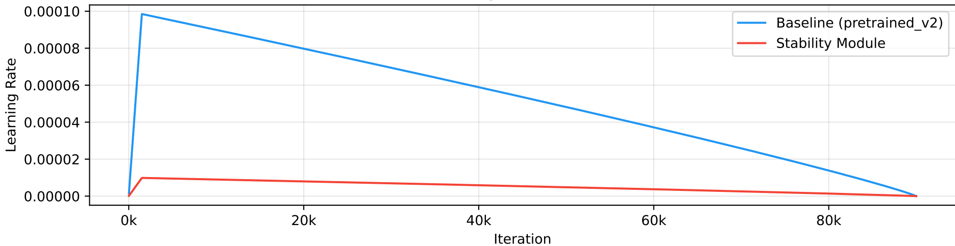
Learning Rate Schedule
