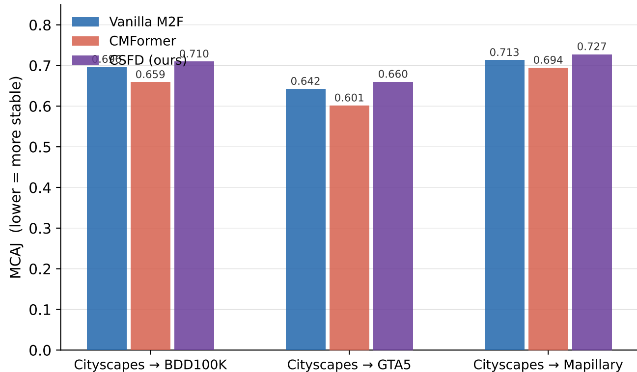
Mean Cross-Attention JSD (MCAJ) by Domain
