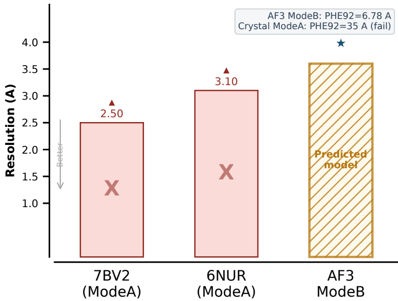
NSP7-NSP8
