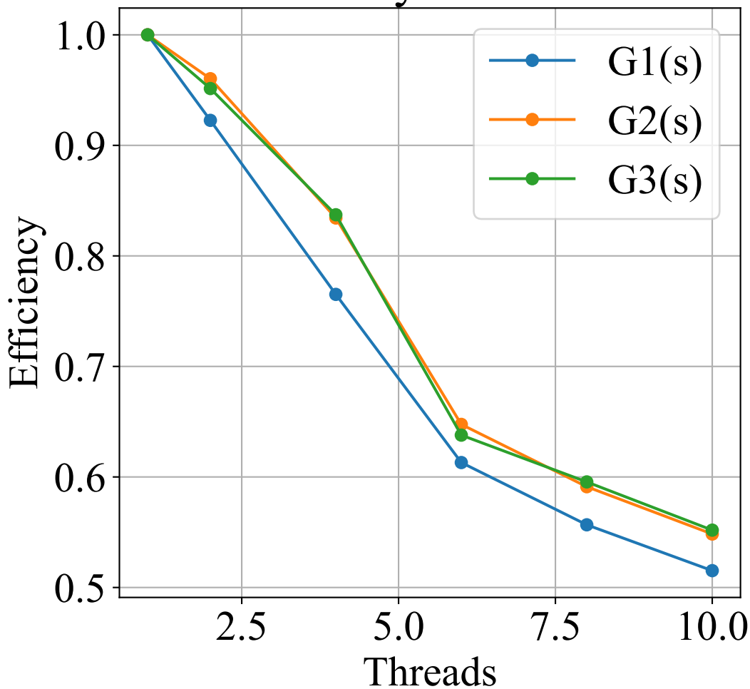
Efficiency vs Threads
