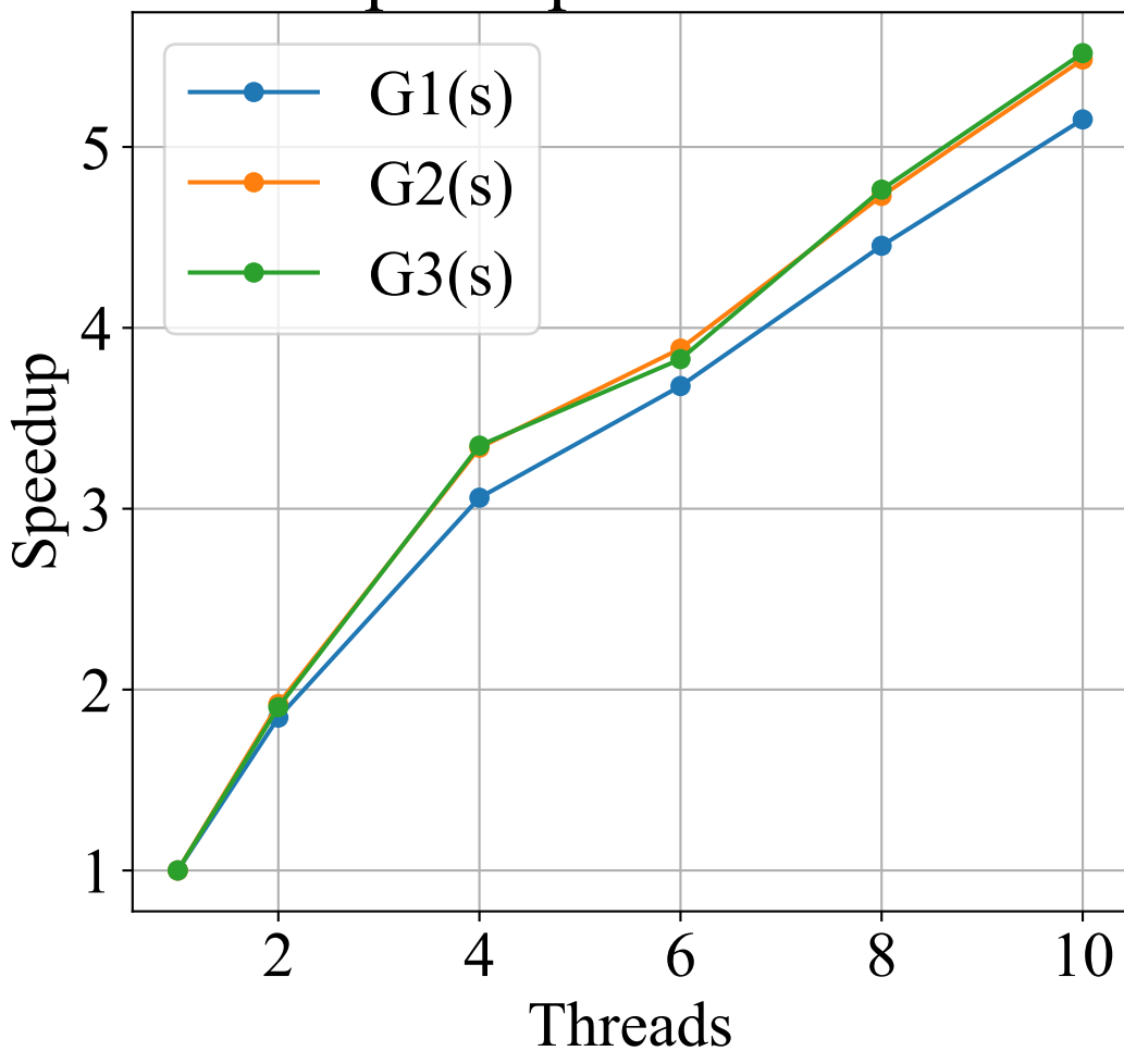
Speedup vs Threads
