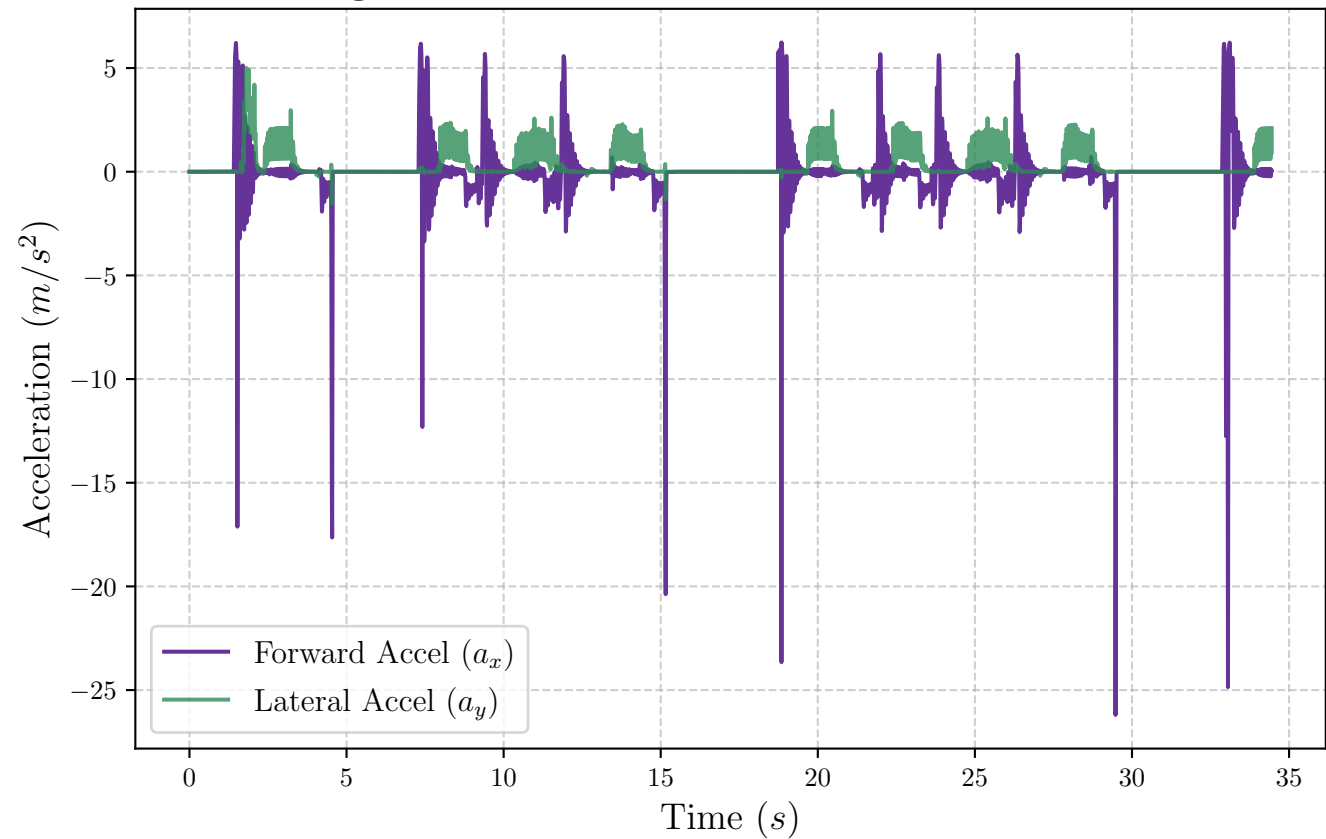
Ego Vehicle Linear Acceleration Over Time
