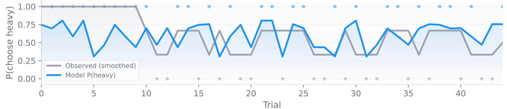
Subject 281 — \omega = 0.56 , \kappa = 0.17
