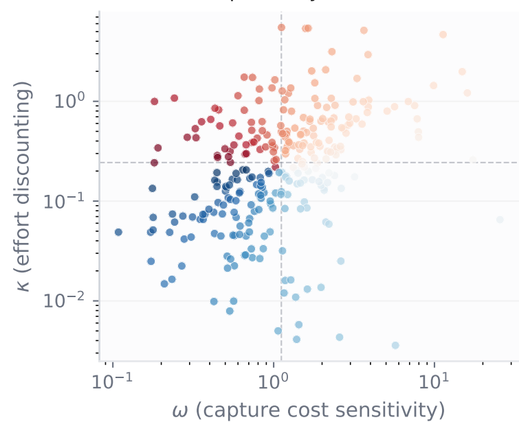
Exploratory (N=290)
