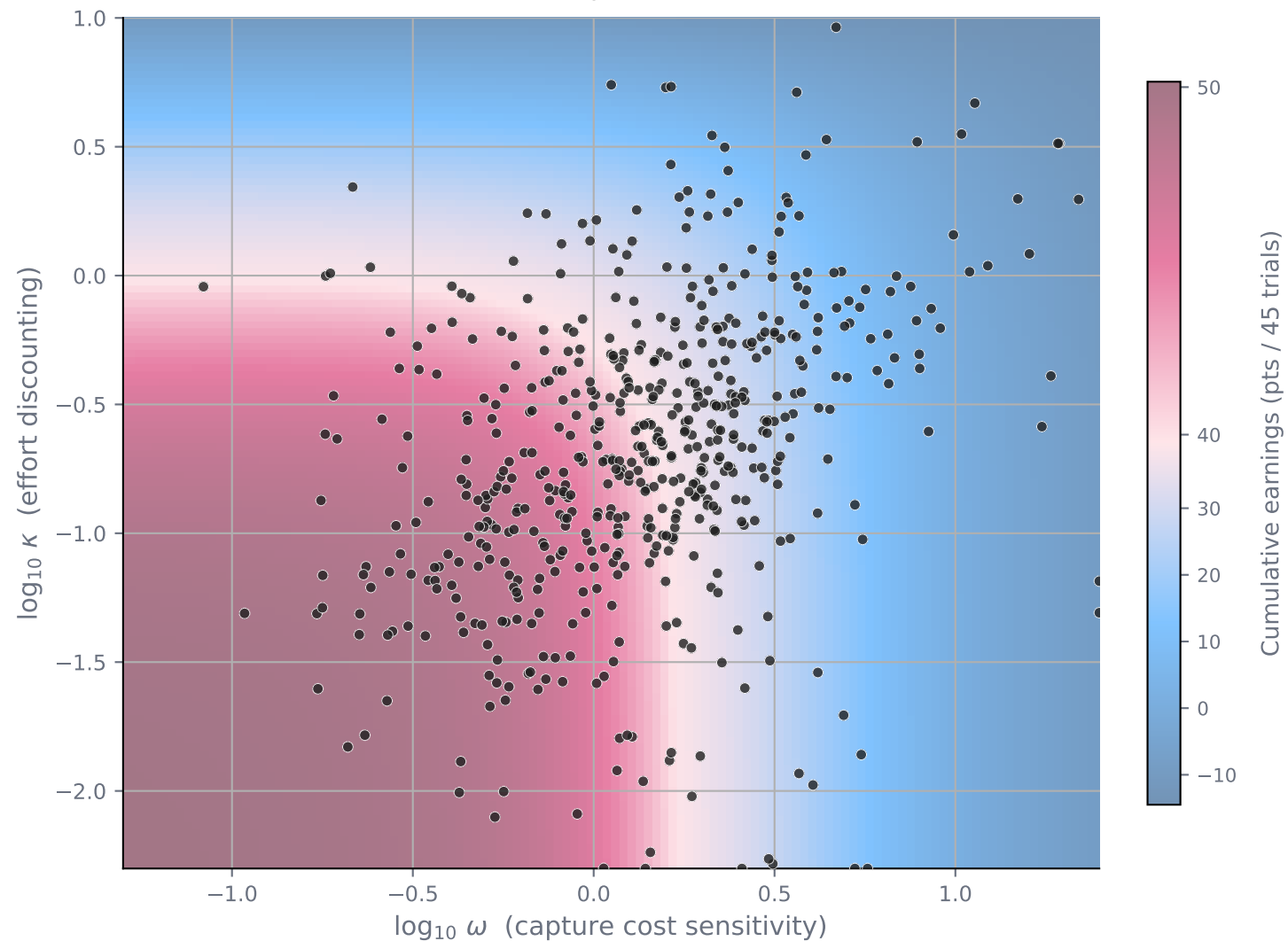
Joint sample (N=571)
