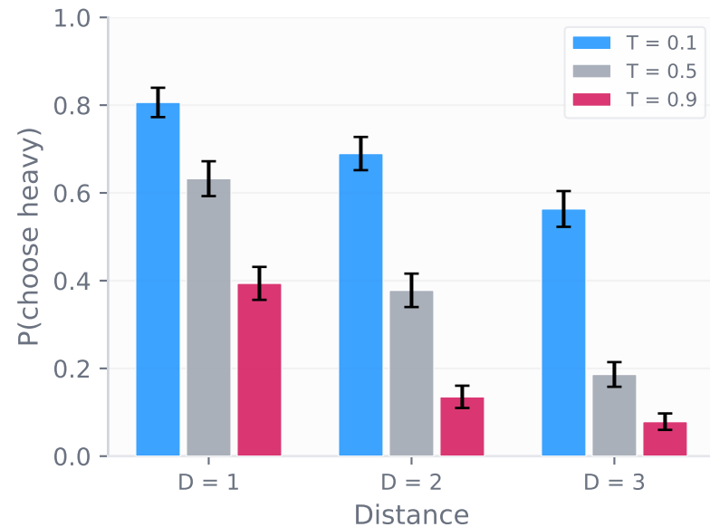
Exploratory (N=290)
