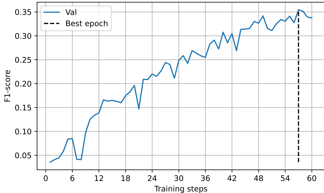
F1-score
