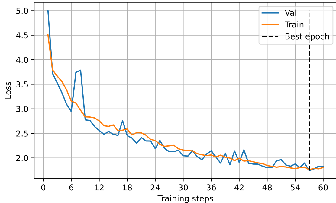
Losses
