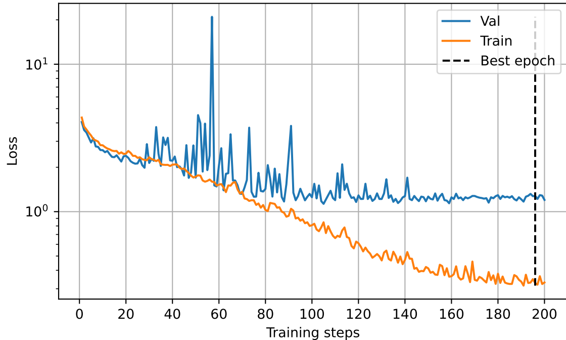
Losses
