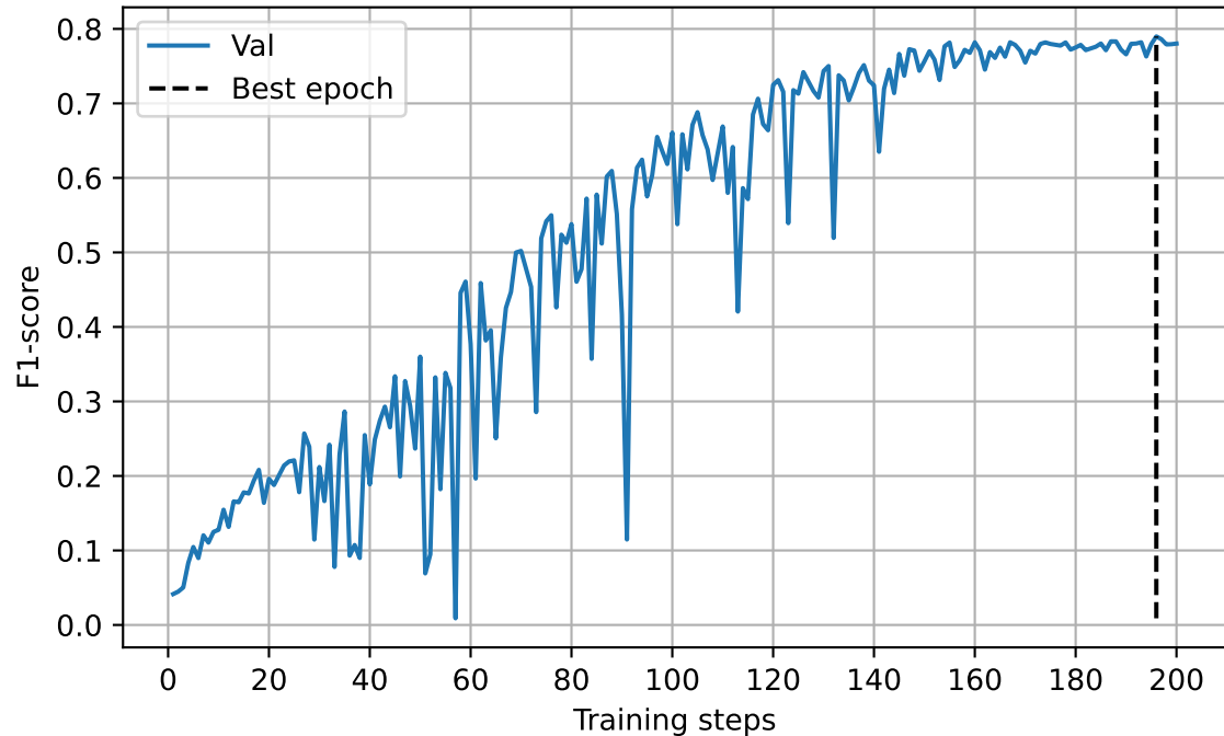
F1-score
