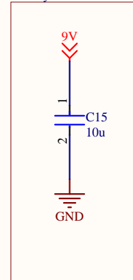
Battery Filter
