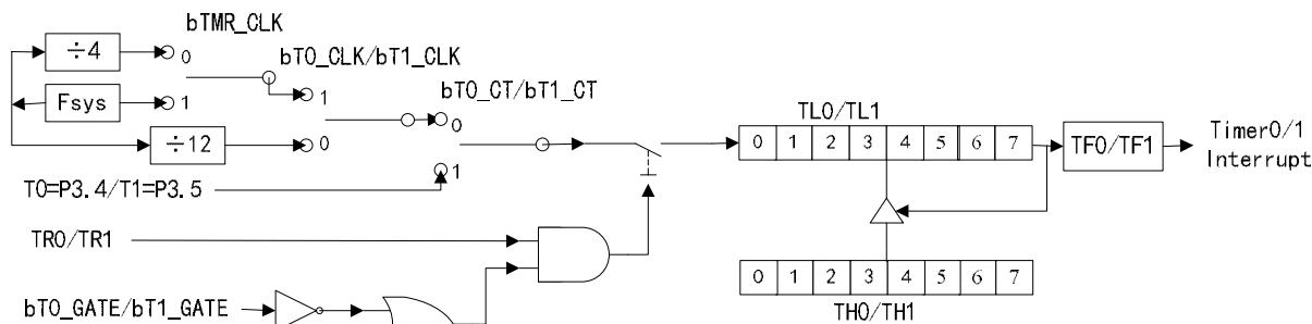
Figure 12.4.1.3 Timer0/1 mode2
