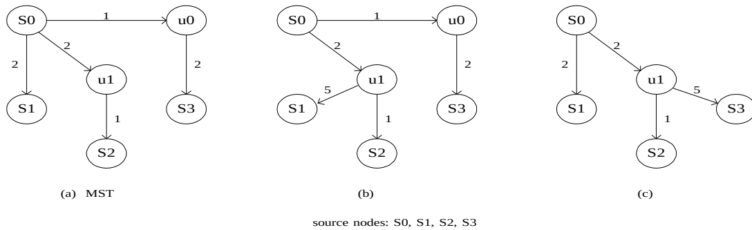
Figure 5 A minimal spanning tree and its first-order neighbor trees.
