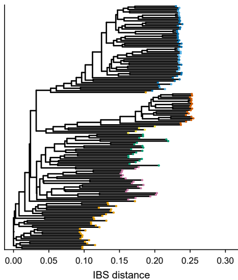
Set 1 (WGS) NJ tree (150 tips)
