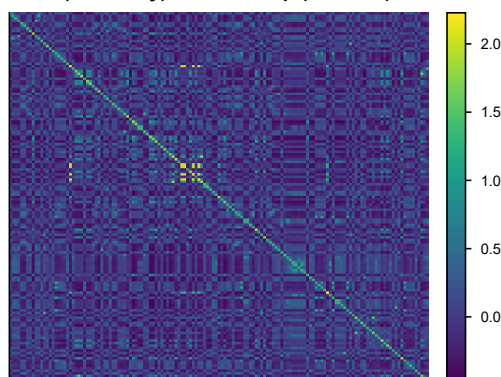
Set 2 (50K array) GRM kinship (147x147)
