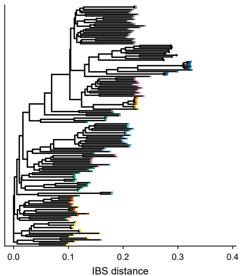
Set 2 (50K array) NJ tree (147 tips)
