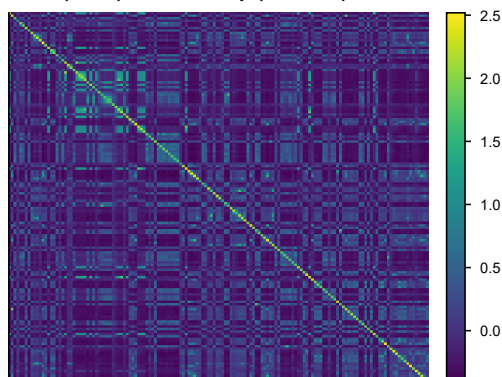
Set 1 (WGS) GRM kinship (150x150)
