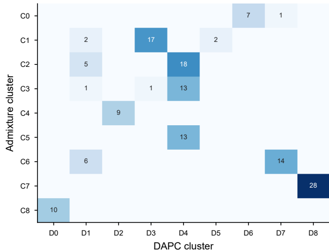
Set 2 (50K array) — ARI = 0.62
