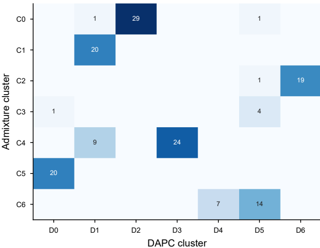
Set 1 (WGS) — ARI = 0.76
