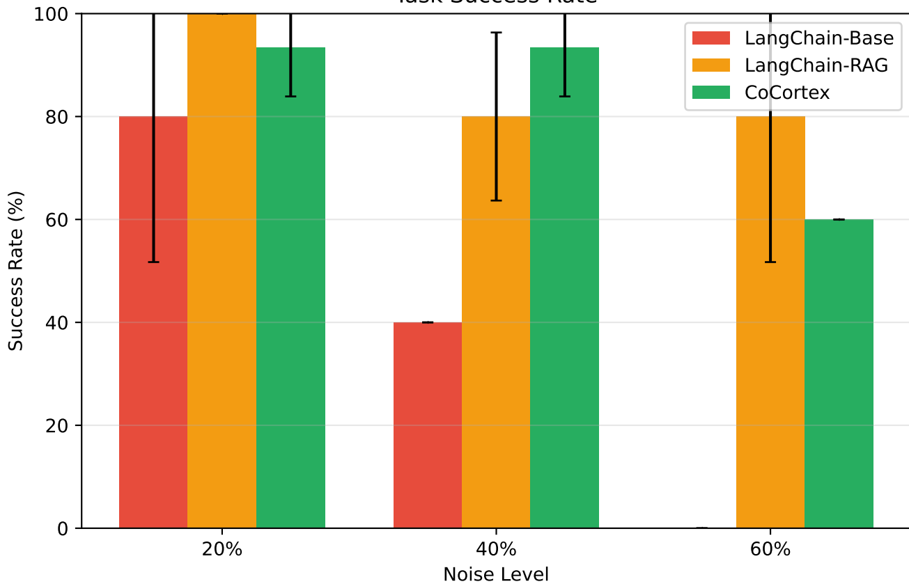
Task Success Rate
