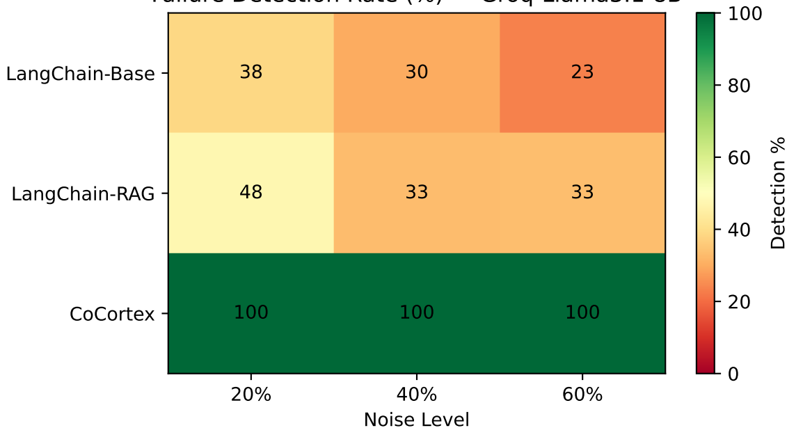
Failure Detection Rate (%) — Groq-Llama3.1-8B
