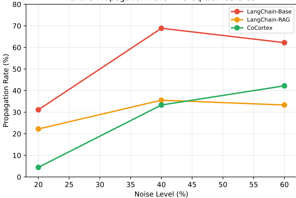
Failure Propagation Rate — Groq-Llama3.1-8B
