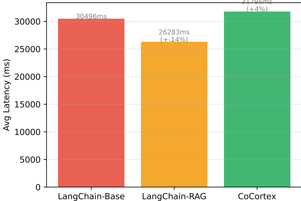
Latency Overhead — Groq-Llama3.1-8B
