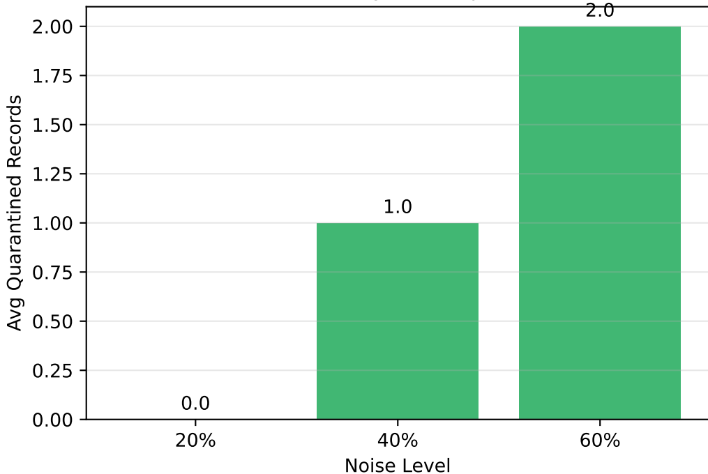
Quarantine Activity — Groq-Llama3.1-8B
