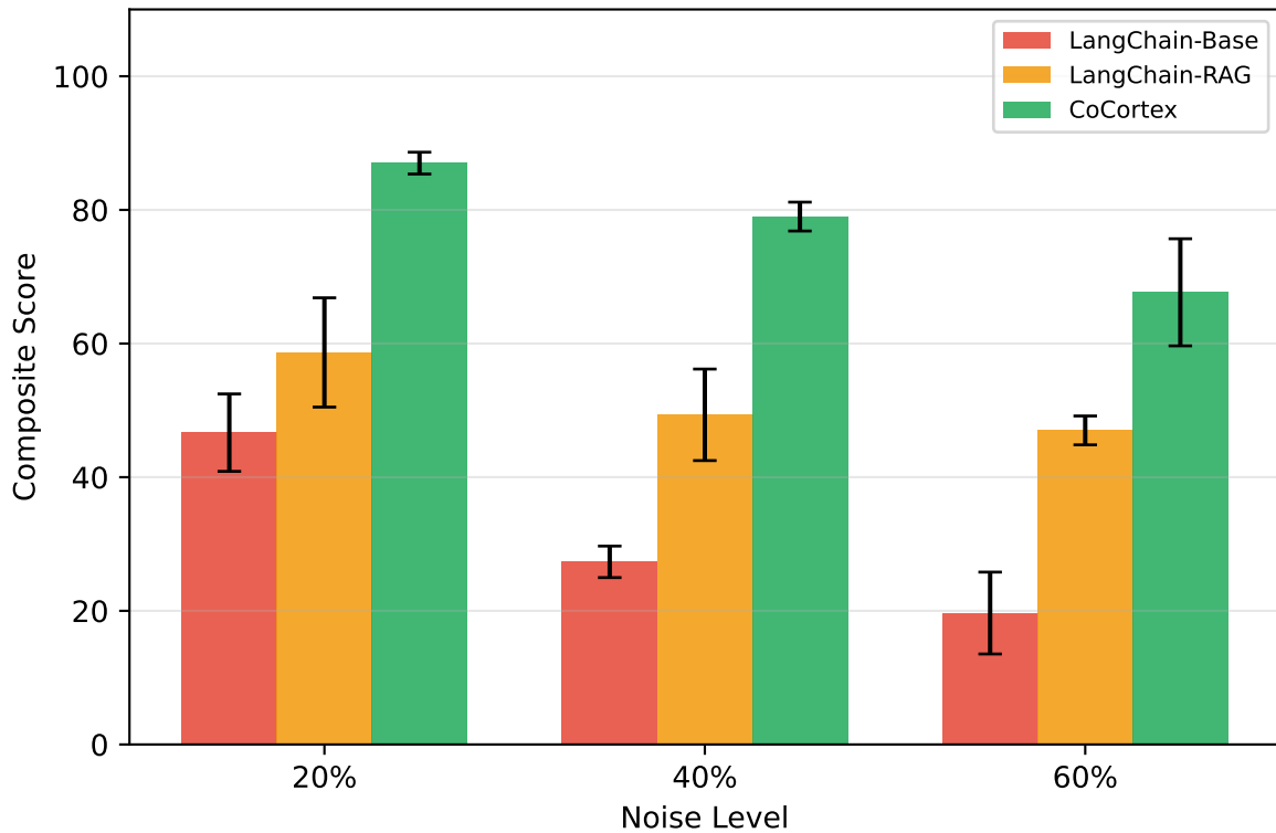
Governance-Aware Score — Groq-Llama3.1-8B
