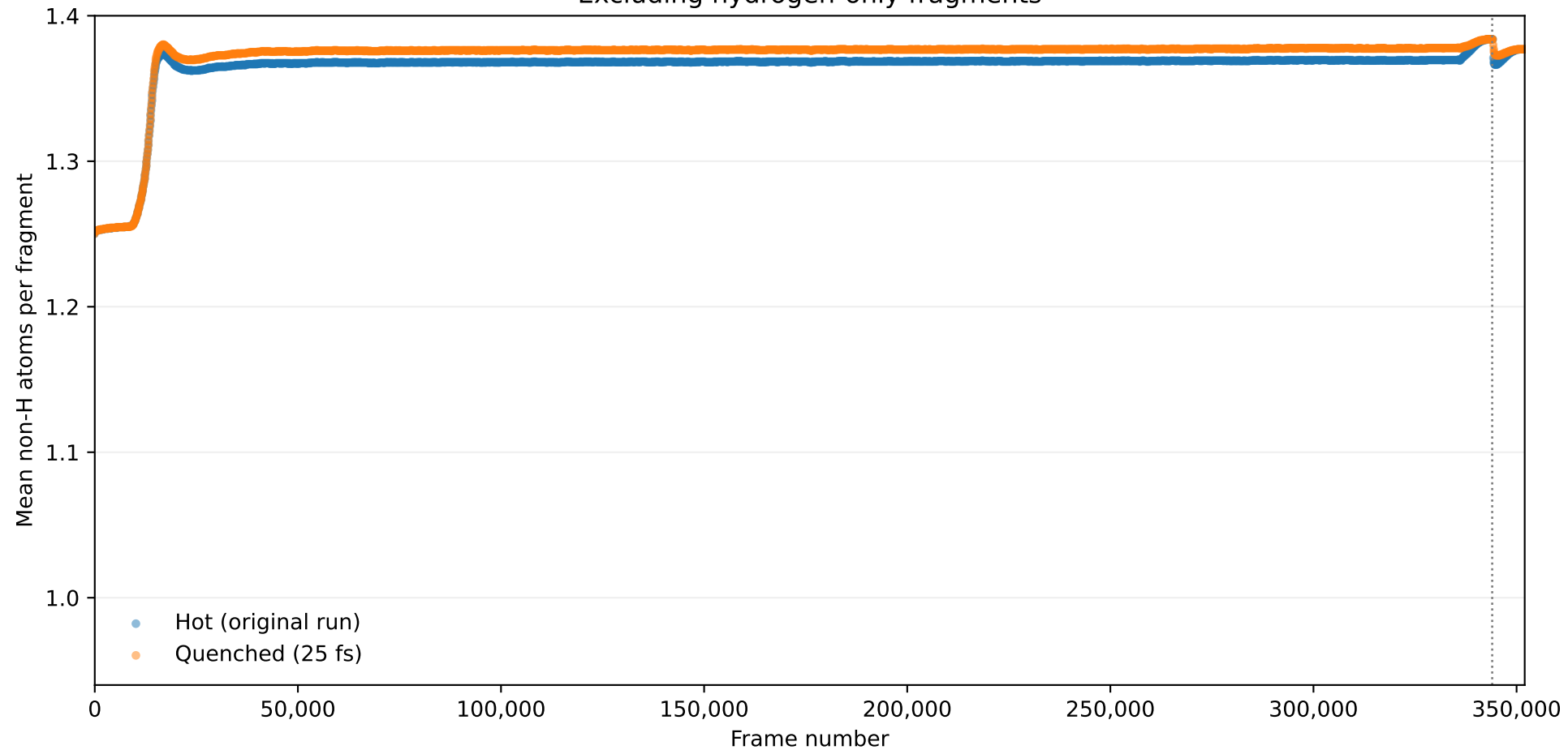
Mean heavy-atom fragment size over the simulation Excluding hydrogen-only fragments
