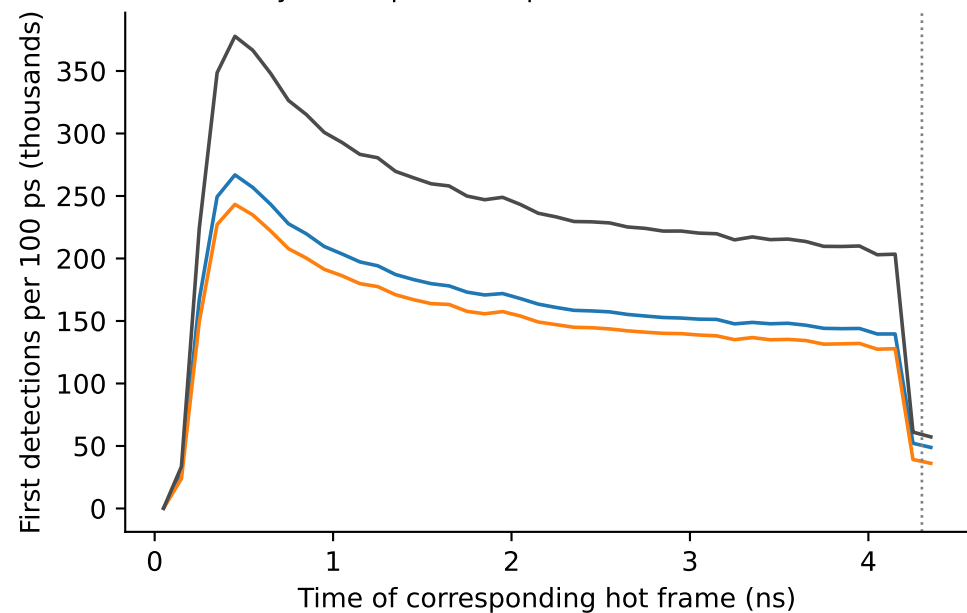
B Discovery in complete 100 ps windows
