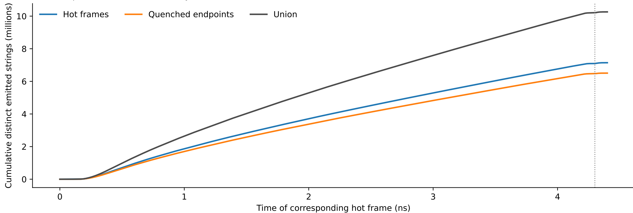
B Discovery in complete 100 ps windows
