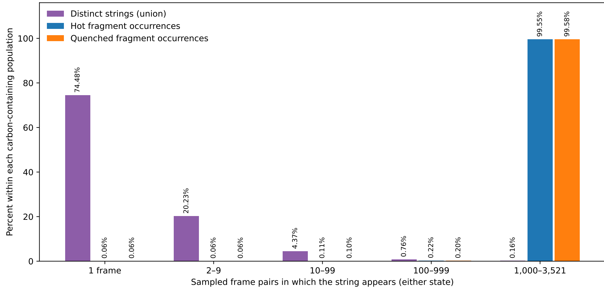
Most string varieties are rare; most occurrences belong to recurrent strings
